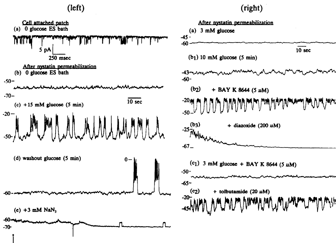
Fig. 1. (Left) Metabolically regulated electrical activity recorded from a cell at the surface of human pancreatic islets using the nystatin permeabilized patch technique. The cell was operationally identified as a B cell by the presence of K^+ (ATP) channels (trace a). Metabolic regulation of V_m is illustrated in traces b–e (see text for full description). (Right) Pharmacological modulation of metabolically regulated electrical activity from another surface human islet cell. (See text for description.)
