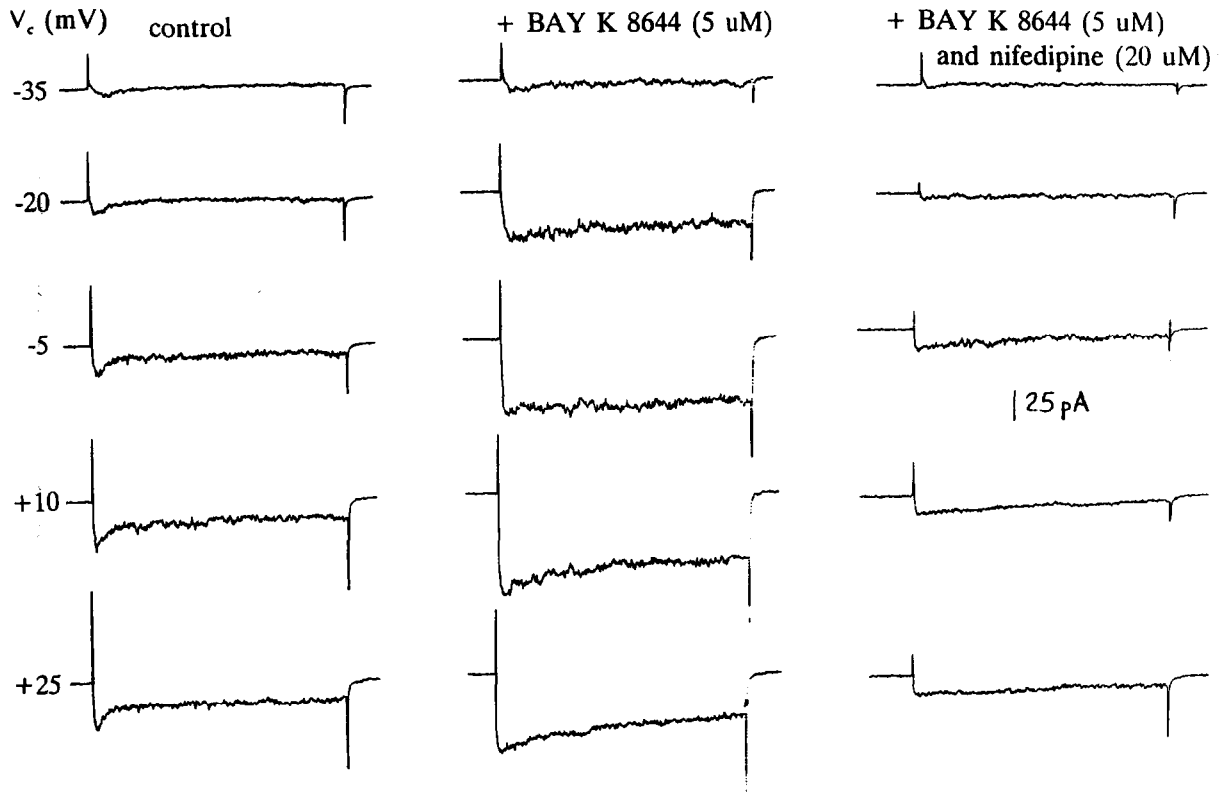
Fig.3. Dihydropyridine-sensitive inward \text{Ca}^{2+} -channel currents recorded on pulsing for 400 ms from a holding potential of -90 mV to indicated clamping potentials. Recording conditions described in the text.
